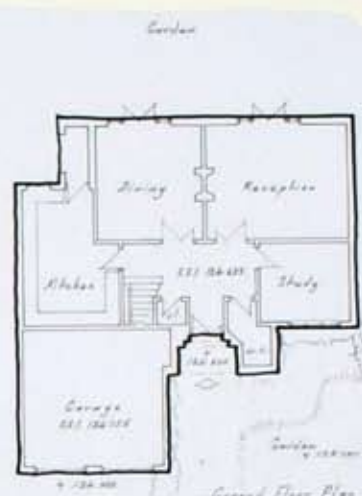
Ground Floor Plan gross floor area: 162 m 2
