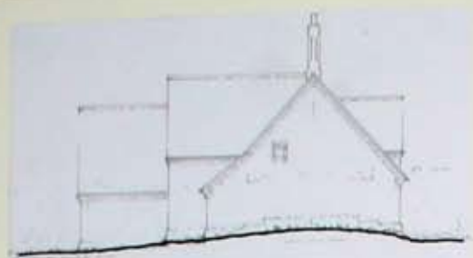
North-West Elevation
